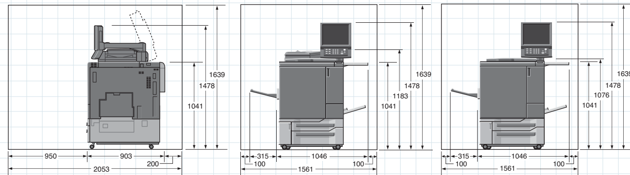
Side View bizhub PRO C1060L+ OT-502+DF-626+MB-506
