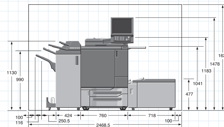
Front View bizhub PRO C1060L+FS-612+DF-626+LU-202+MB-506
