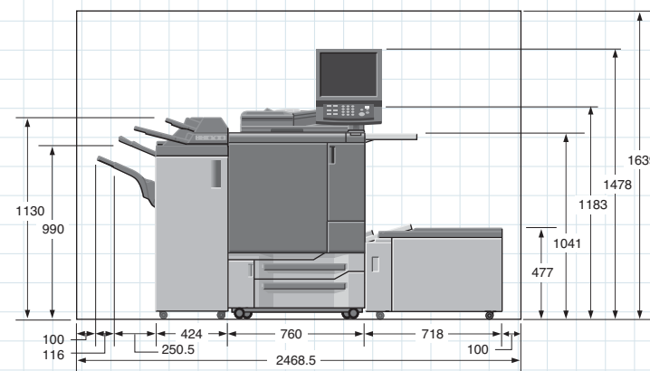
Front View bizhub PRO C1060L+FS-626+LU-202+MB-506
